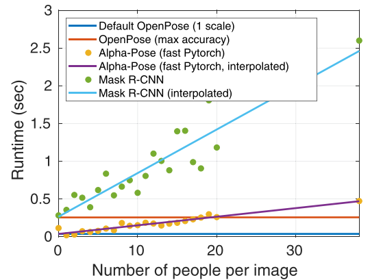
Fig. 12. Inference time comparison between OpenPose, Mask R-CNN, and Alpha-Pose (fast Pytorch version). While OpenPose inference time is invariant, Mask R-CNN and Alpha-Pose runtimes grow linearly with the number of people. Testing with and without scale search is denoted as “max accuracy” and “1 scale”, respectively. This analysis was performed using the same images for each algorithm and a batch size of 1. Each analysis was repeated 1000 times and then averaged. This was all performed on a system with a Nvidia 1080 Ti and CUDA 8.
